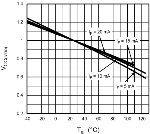
Fig. 12.8 V_{OC(ratio)} - T_a
