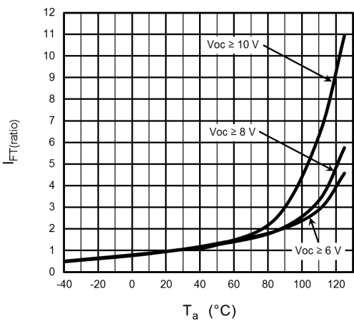
Fig. 12.4 I_{FT}(\text{ratio}) - T_a
