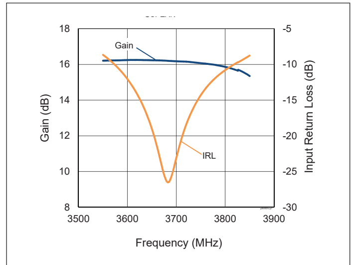
Figure 6. Small Signal CW Gain &amp; Input Return Loss
