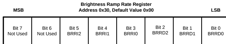
Figure 43. Brightness Ramp Rate Register
