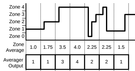
Figure 28. Averager Calculation
