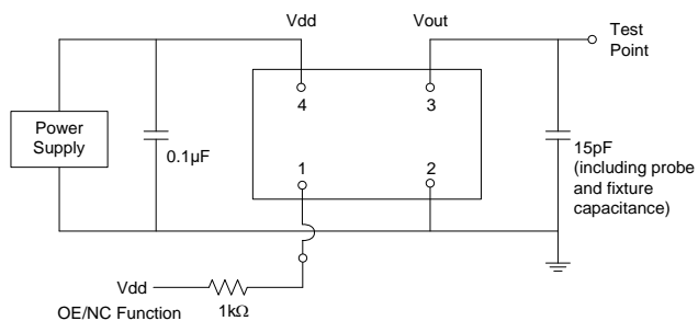
Figure 2. Test Circuit [6]
