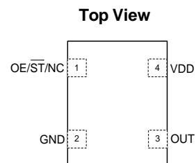
Figure 1. Pin Assignments
