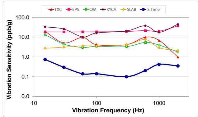
Figure 16. Vibration Robustness [5]
