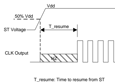
Figure 5. Standby Resume Timing (ST Mode Only)
