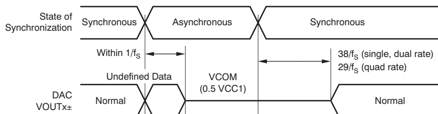
Figure 36. DAC Outputs During Loss of Synchronization
