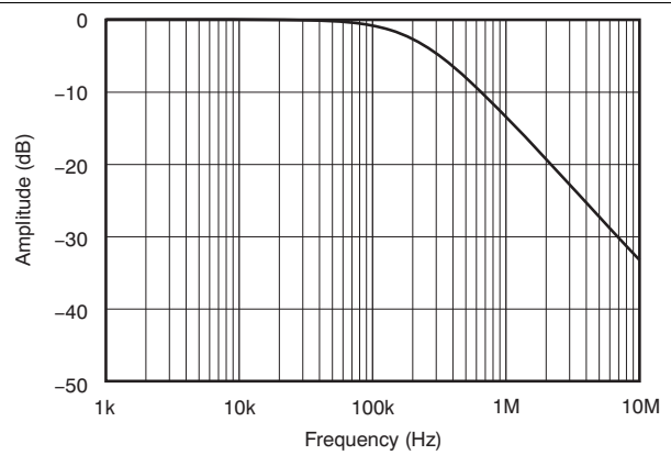
Figure 9. De-emphasis Characteristic
