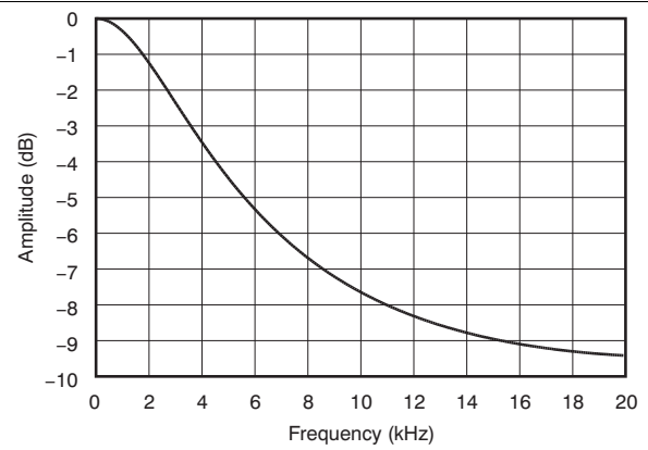
Figure 9. De-emphasis Characteristic
