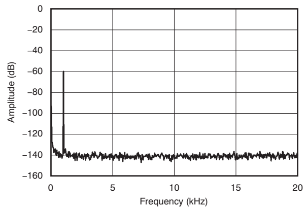
Figure 17. Output Spectrum
