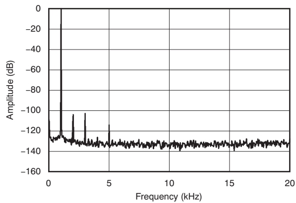
Figure 16. Output Spectrum
