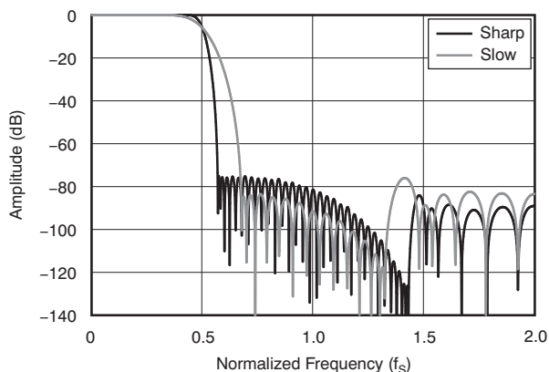
Figure 4. Frequency Response (Dual Rate)
