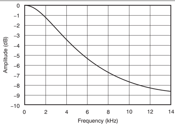
Figure 8. De-emphasis Characteristic
