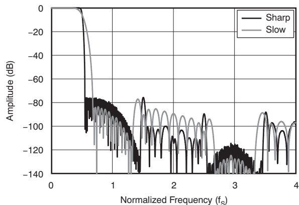
Figure 2. Frequency Response (Single Rate)
