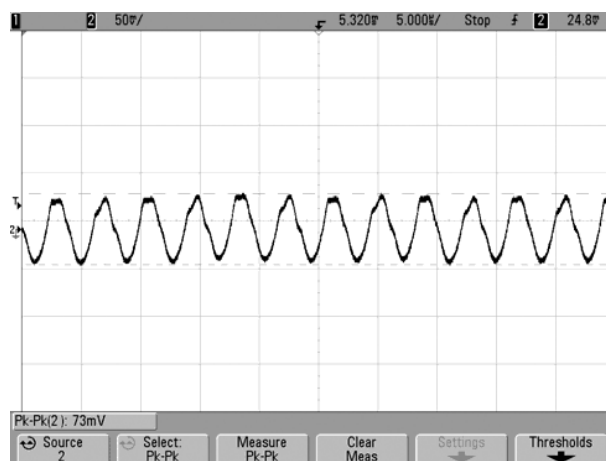
Output Ripple and Noise (Vin=75V, Iout=25A, Load=0, Ta=+25°C., ScopeBW=20MHz)
