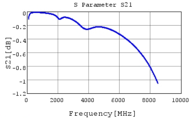
GRM2165C2A101JA01 S21 DCOV, 25degC
