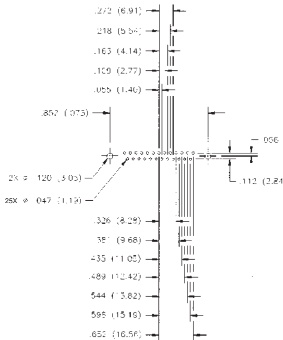
25 Position Shell Size B
