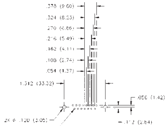
15 Position Shell Size A
