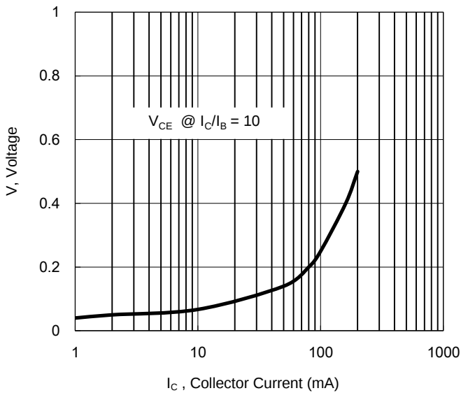
Fig.11 "ON" Voltages
