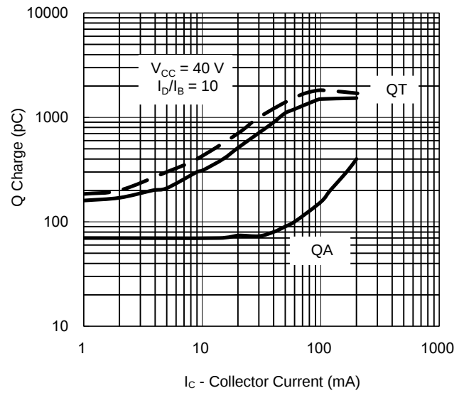
Fig.2 Charge Data
