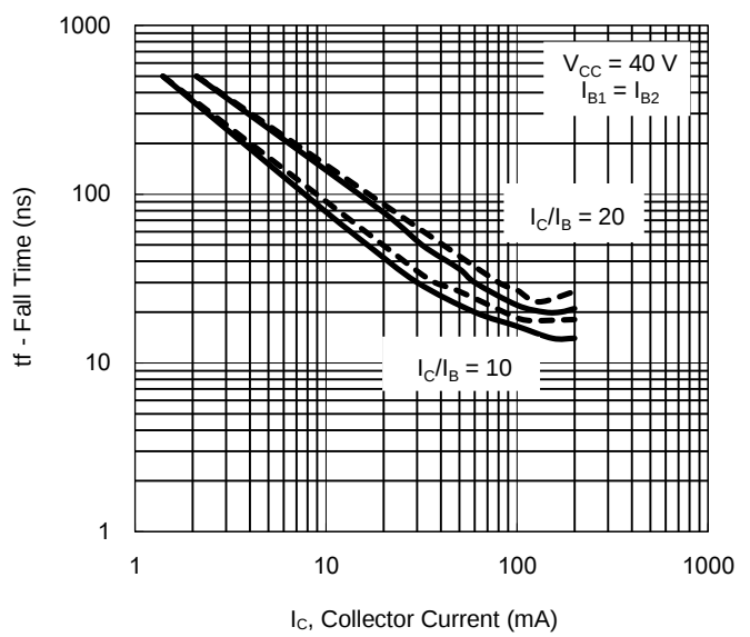
Fig.4 Fall Time
