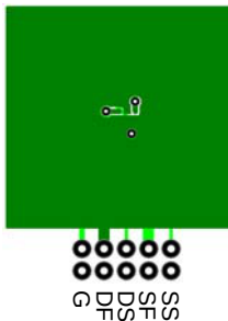
a. 52\text{ }^{\circ}\text{C}/\text{W} when mounted on a 1 in 2 pad of 2 oz copper
