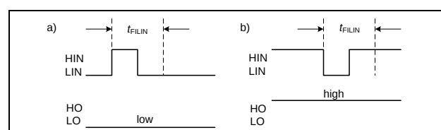
Figure 4 Input filter timing diagram
