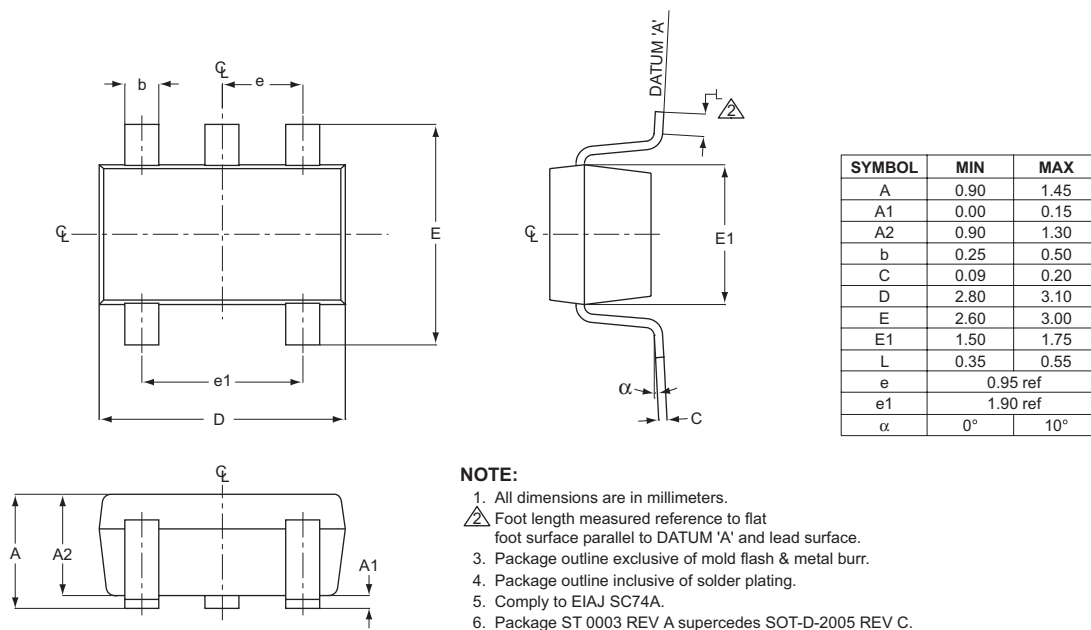
Figure 51. SOT23-5 Package
