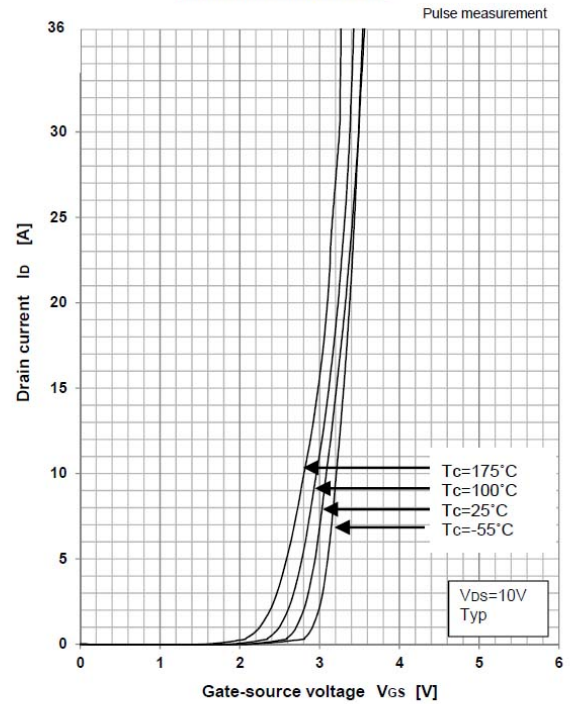
Transfer characteristics
