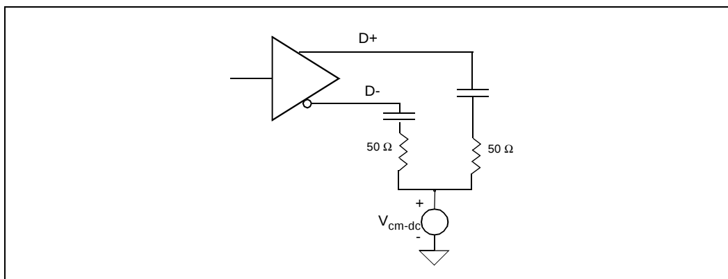
Figure 22. Transmitter Test Load (100 Ω diff Load)
