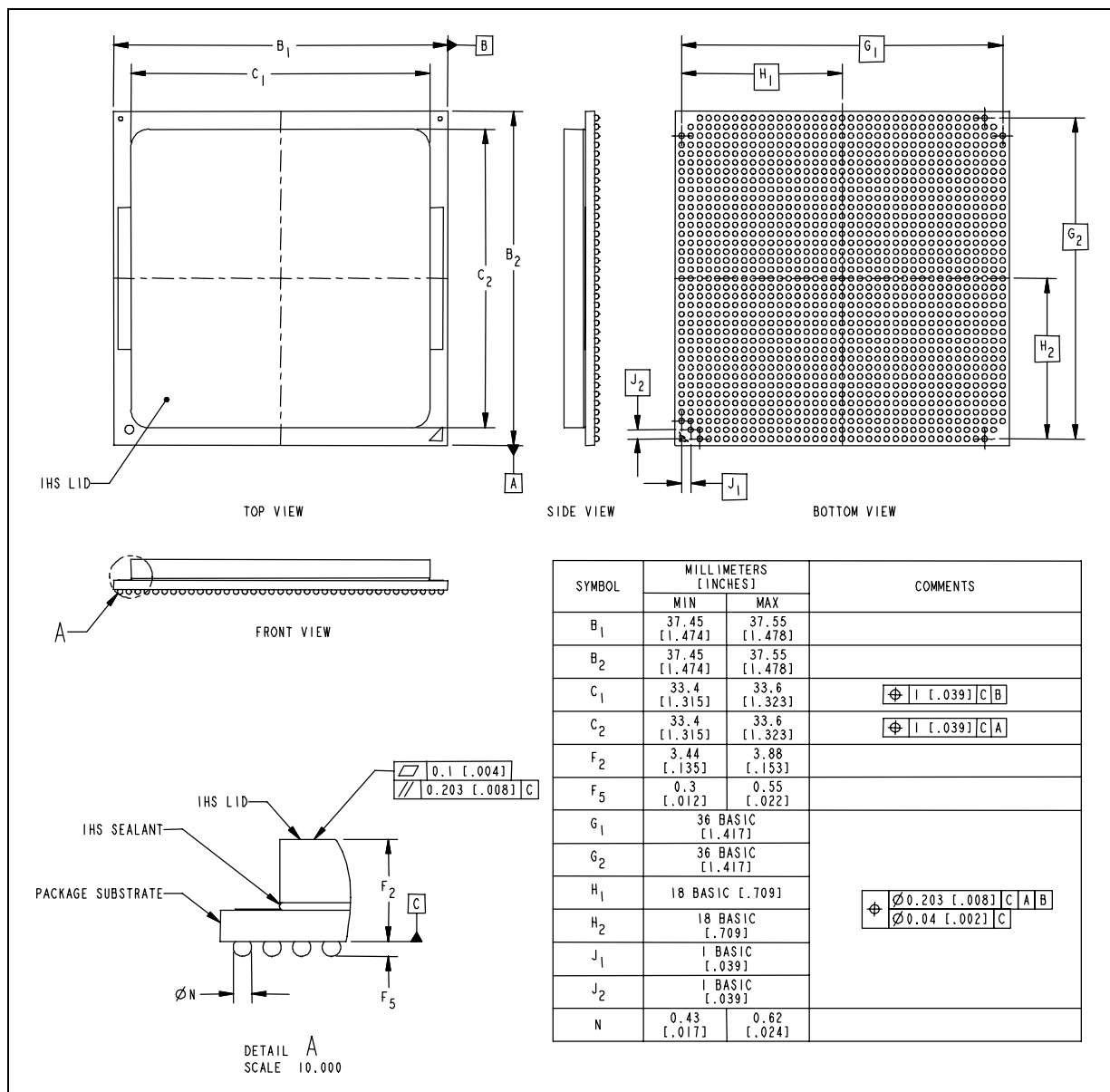
Figure 3. 1357-Lead FCBGA Package (Top and Bottom Views)
