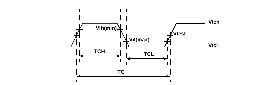
Figure 10. Clock Timing Measurement Waveforms
