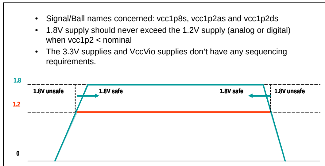
Figure 27. Intel® 81341 and 81342 I/O Processors 1.2V/1.8V Power Sequencing System Requirements
