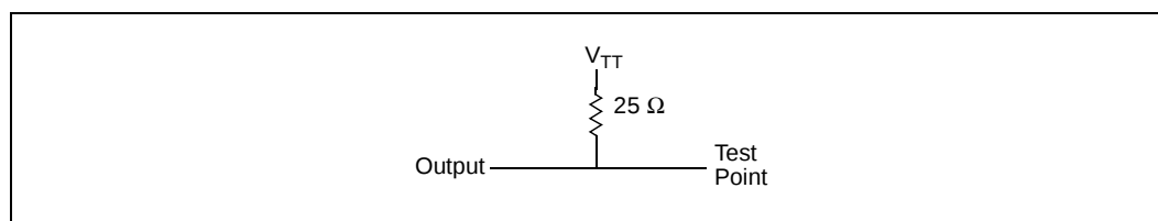
Figure 18. AC Test Load for DDR2 SDRAM Signals
