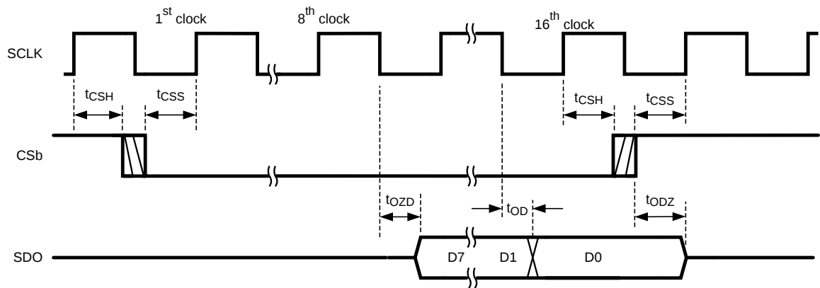
Figure 55. Read Timing
