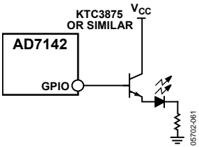
Figure 45. Controlling LEDs Using the GPIO
