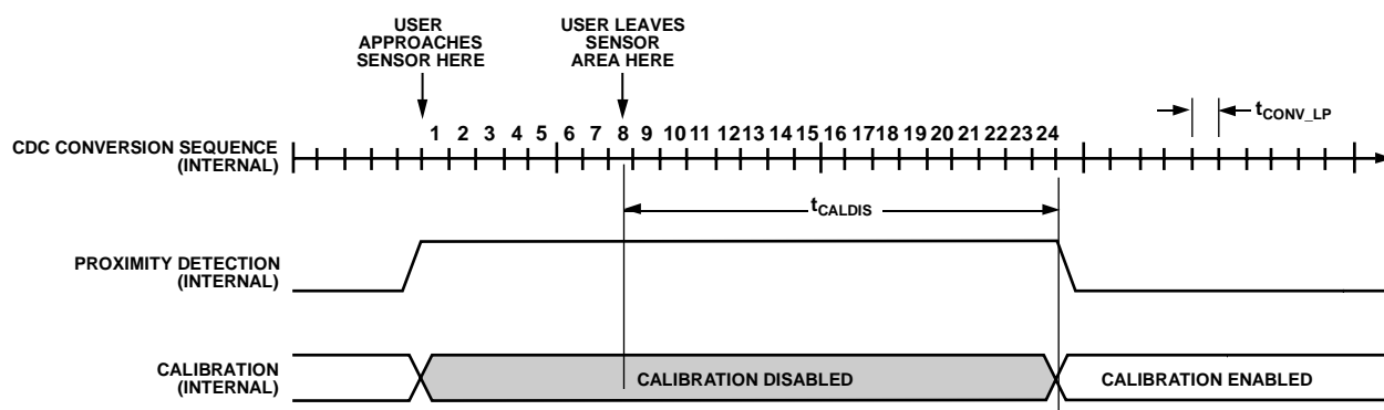
Figure 28. Full Power Mode Proximity Detection Example with FP\_PROXIMITY\_CNT = 1
