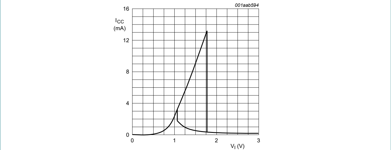
Fig. 15. Typical 74LVC1G98 transfer characteristic; V_{CC} = 3.0 V
