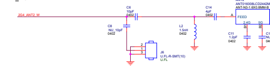
Figure 6-1. Schematic
