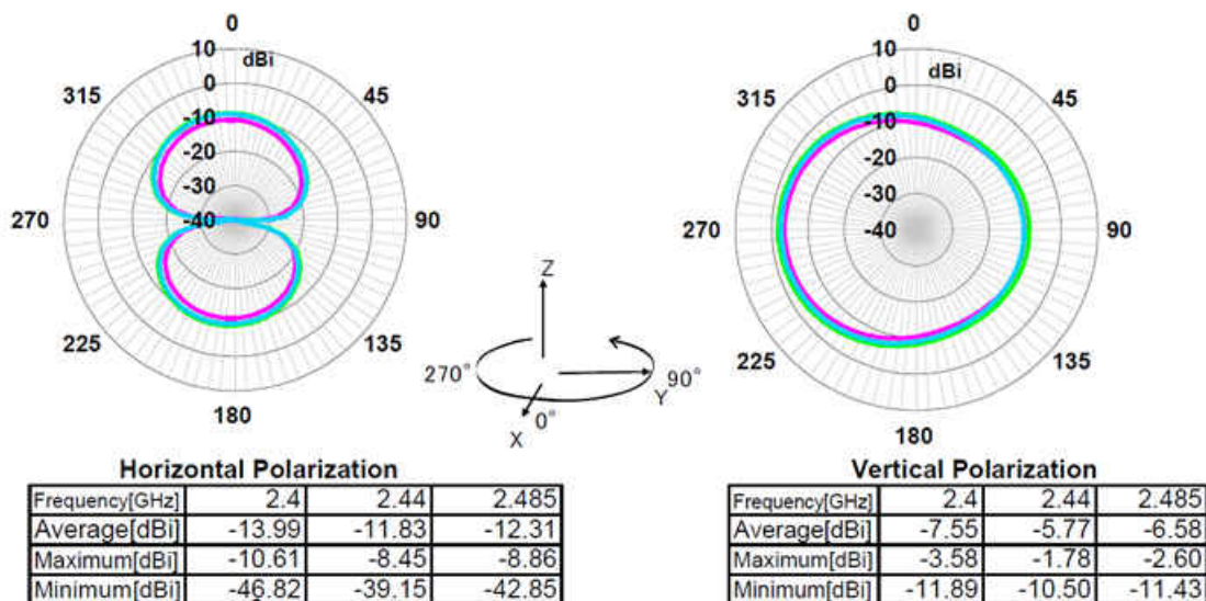
Figure 5-9. ANT2 Polarization
