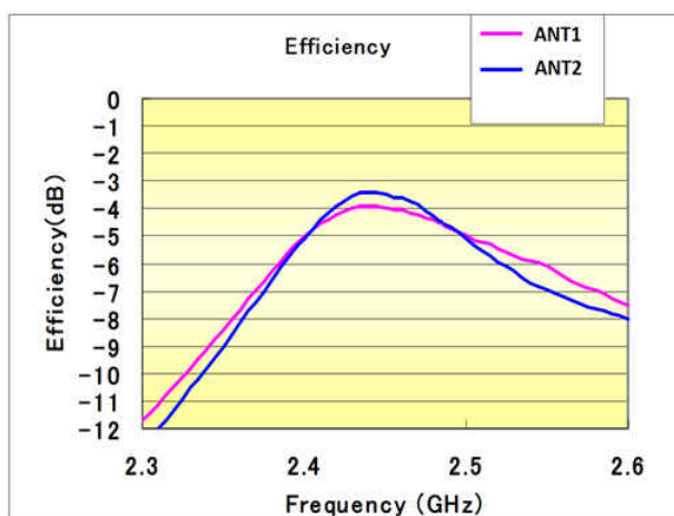
Figure 5-2. Antenna Efficiency
