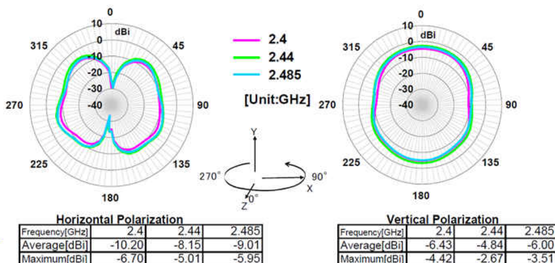
Figure 5-7. ANT2 Polarization
