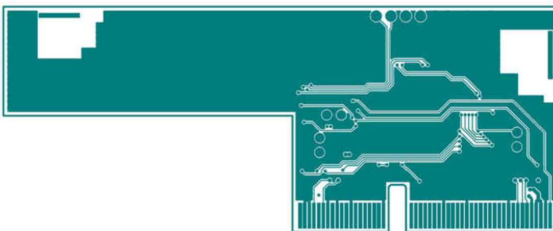
Figure 7-4. Layer 4
