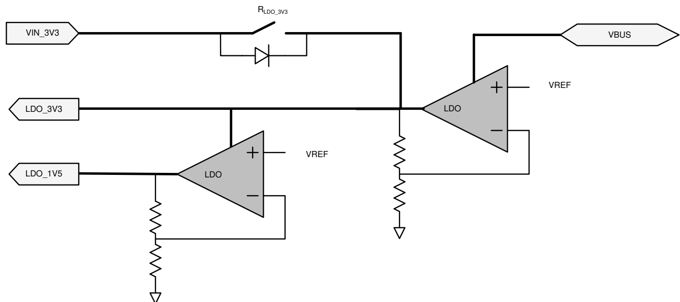
Figure 8-11. Power Supplies
