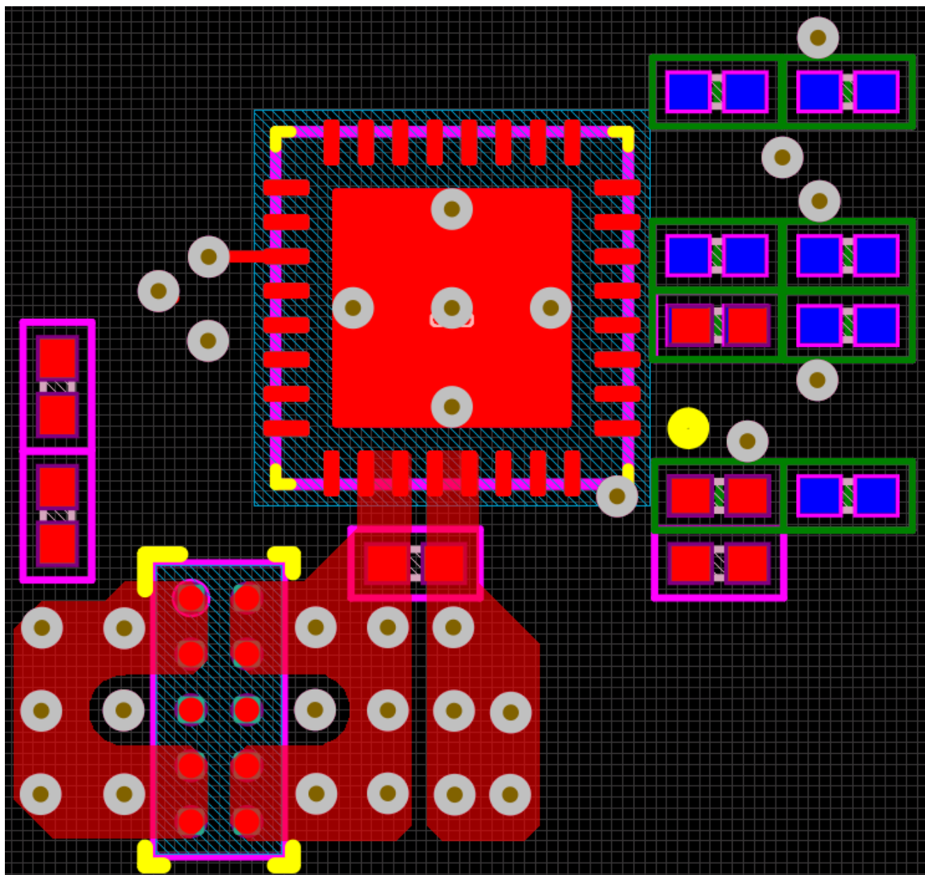
Figure 9-26. VBUS Copper Pours and Via Placement
