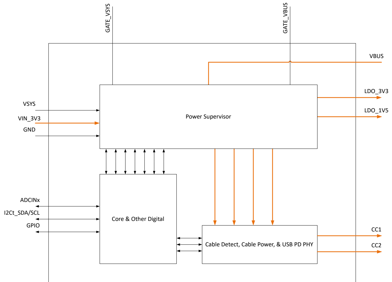
Figure 8-2. TPS25730S
