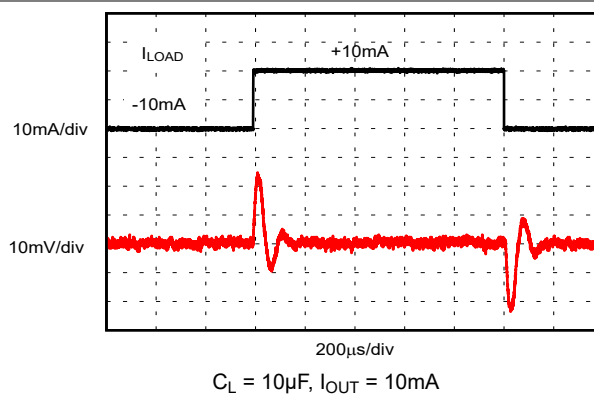
Figure 6-20. Load Transient
