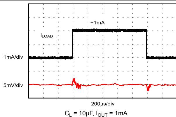
Figure 6-19. Load Transient
