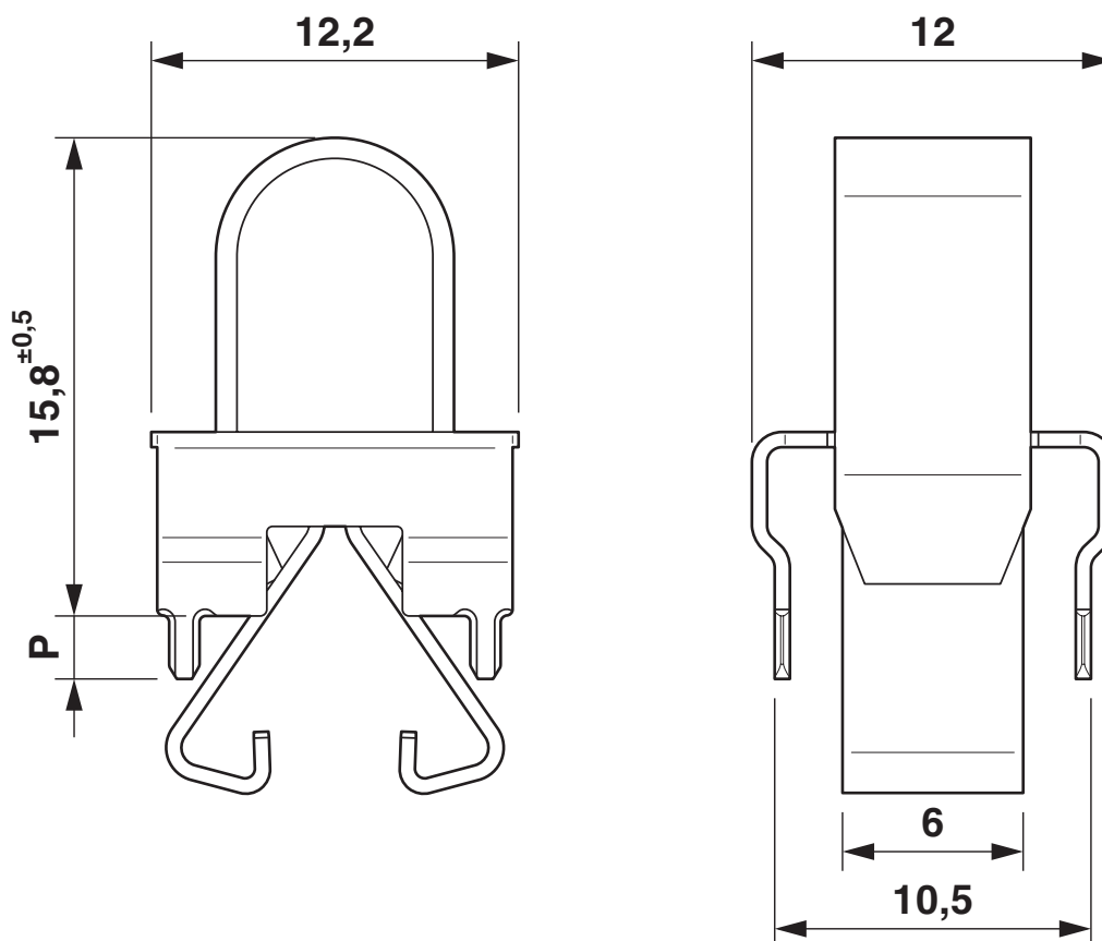
Dimensional drawing
