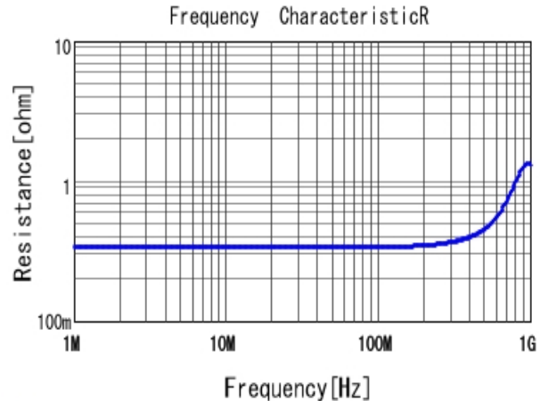
■ DE11XRA220KJ4BQ01F R DC0V, 20degC
