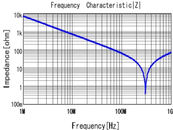
■ DE11XRA220KJ4BQ01F |Z| DC0V, 20degC
