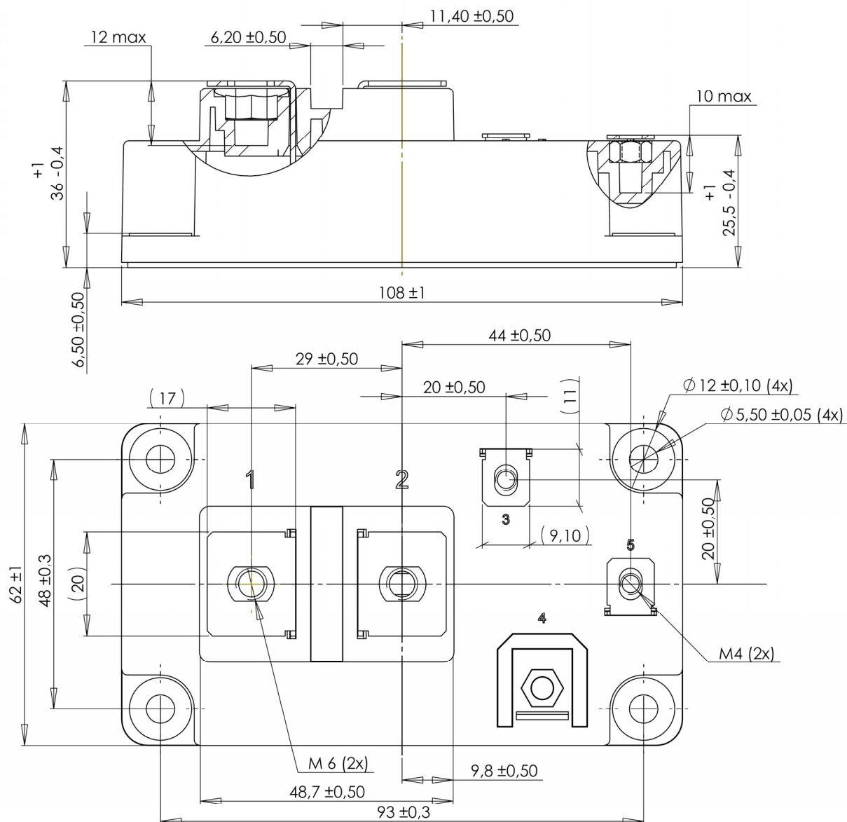
D4 Package outline (dimensions in mm)
