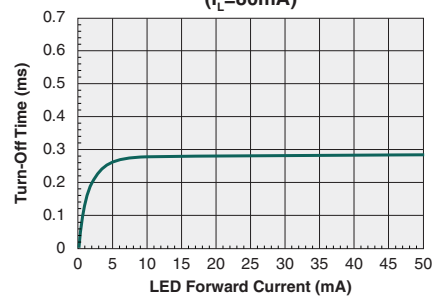
Turn-Off Time vs. LED Forward Current ( I_L=80\text{mA} )
