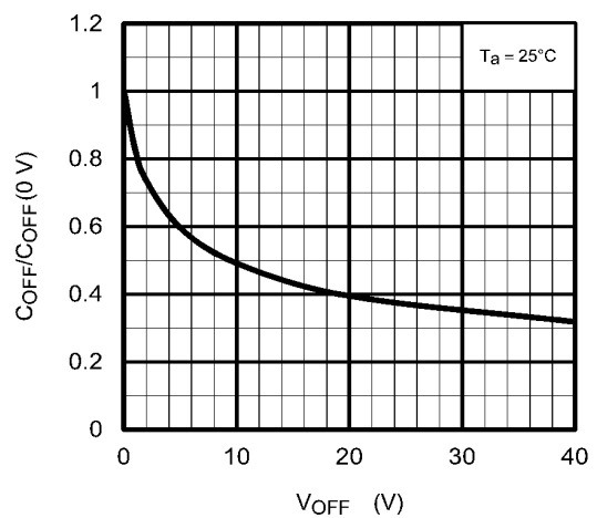
Fig. 12.1.11 C_{OFF}/C_{OFF}(0\text{ V}) - V_{OFF}
