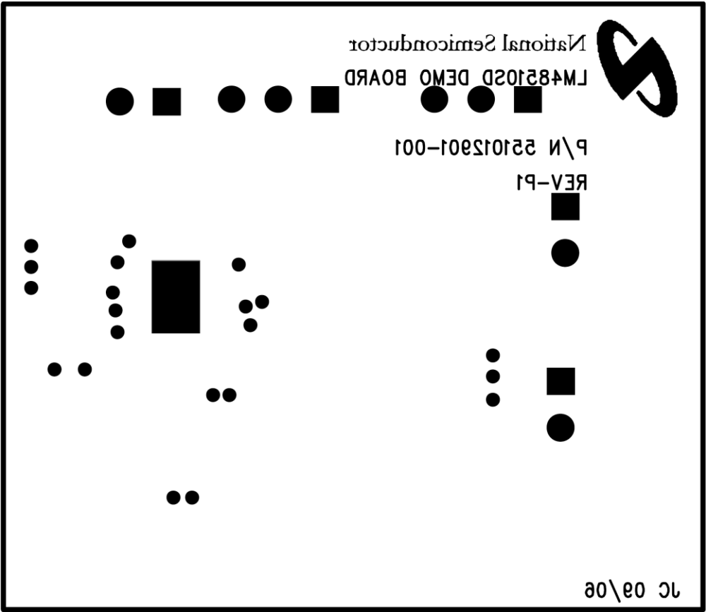
Figure 36. Bottom Silkscreen
