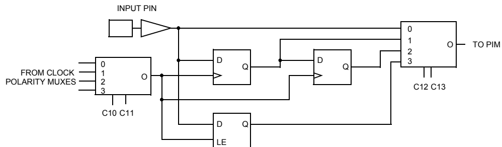
Figure 9. Input Macrocell
