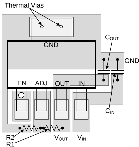
Figure 33. LP38692-ADJ SOT-223 Package
