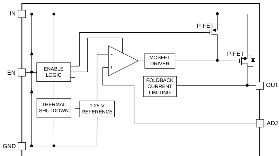
Figure 28. LP38692-ADJ (SOT-223, WSON)
