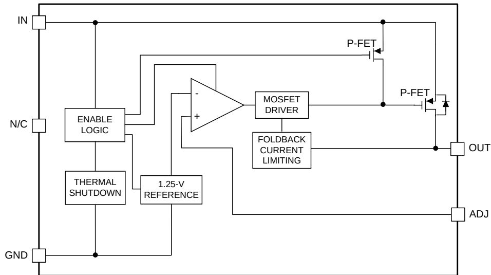
Figure 27. LP38690-ADJ (WSON)
