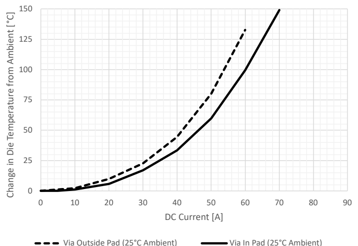
Figure 16: Comparison with and without In-Pad Vias at Ambient Temperature, LC Package
