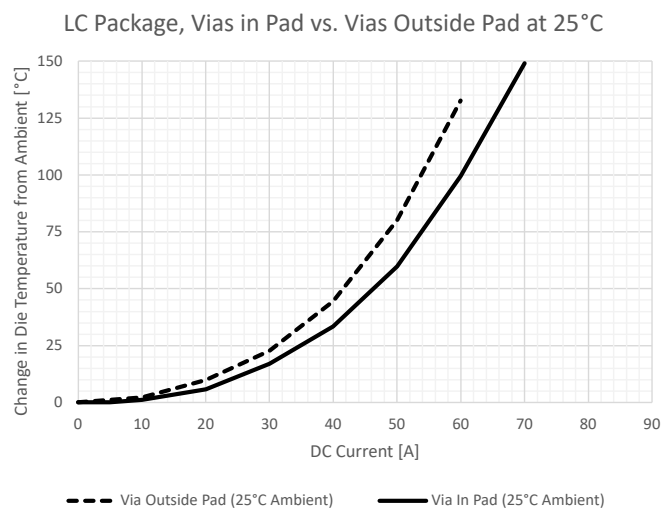
Figure 18: Comparison at 125°C and 25°C, In-Pad Vias, LC Package
