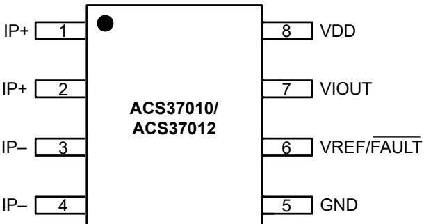
Pinout Diagram Package LC, 8-Pin SOIC
