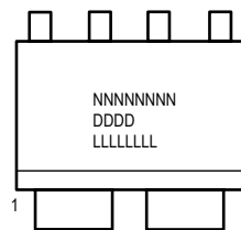
Figure 21: Custom 6-Pin SOIC (Suffix LZ)
