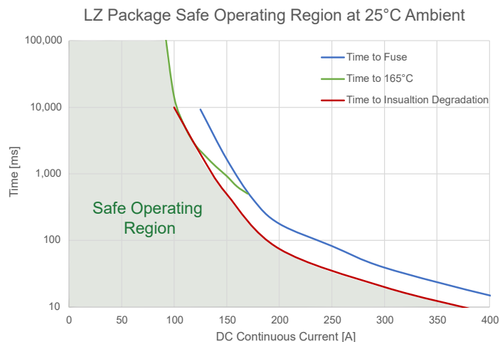
Figure 19: Safe Operating Region, LZ Package
