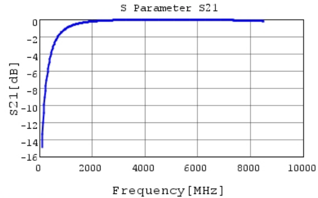
GCQ1555C1H2R9WB01 S21 DCOV, 25degC
