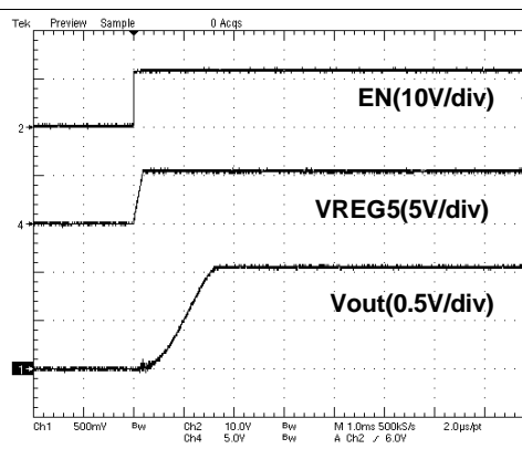
Figure 13. Start-Up Waveform
