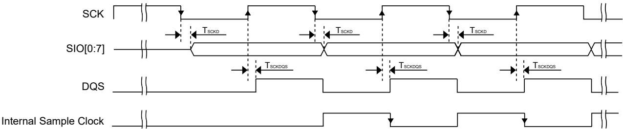
Figure 23. FlexSPI input timing in SDR mode where FlexSPIn_MCR0[RXCLKSRC] = 0X3 (case A2)
