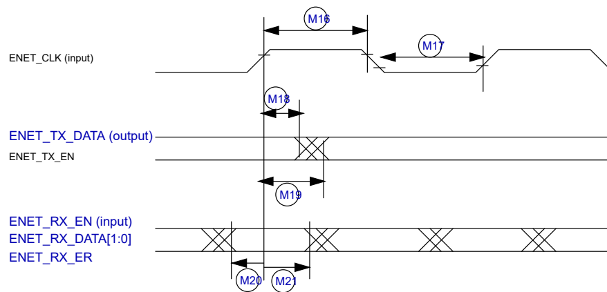
Figure 50. RMII mode signal timing diagram
