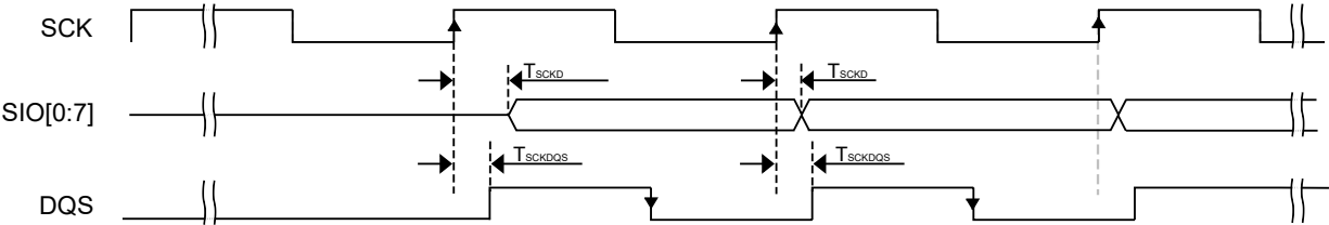
Figure 22. FlexSPI input timing in SDR mode where FlexSPIn_MCR0[RXCLKSRC] = 0X3 (case A1)
