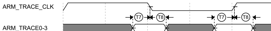
Figure 16. Trace data specifications
