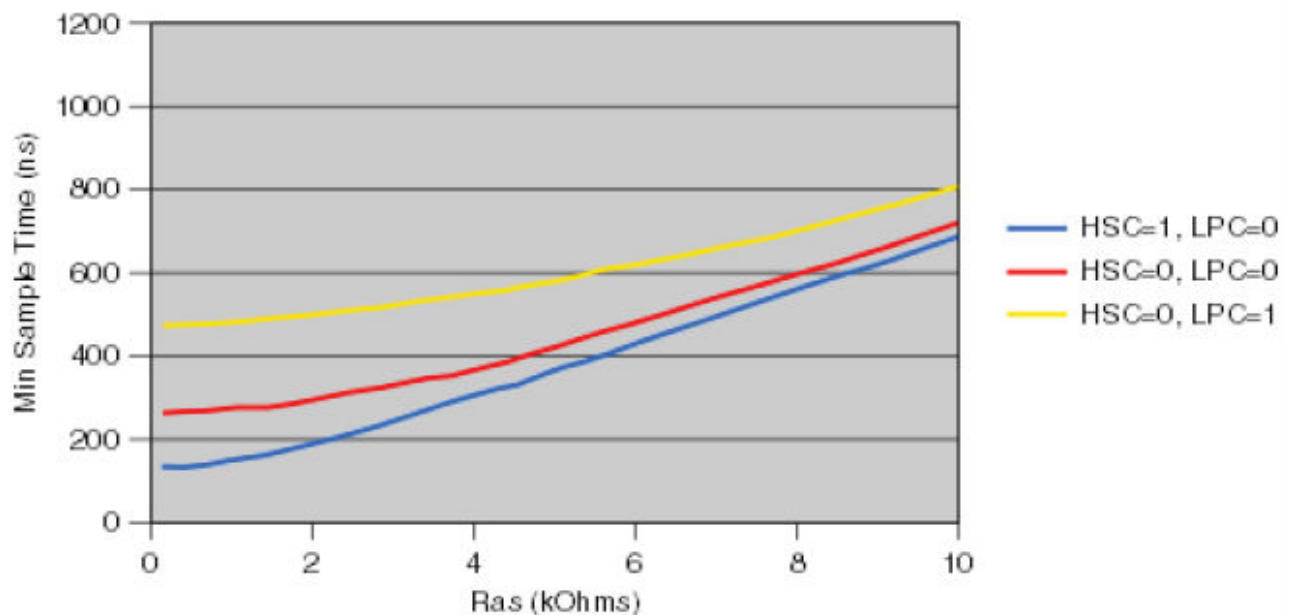
Figure 35. Minimum Sample Time Vs Ras (Cas = 2pF)
