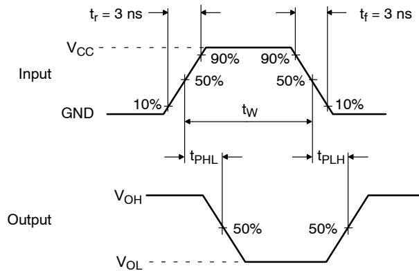
Figure 6. AC Waveforms
