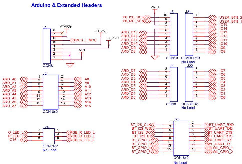
Figure 4-10. I/O Headers
