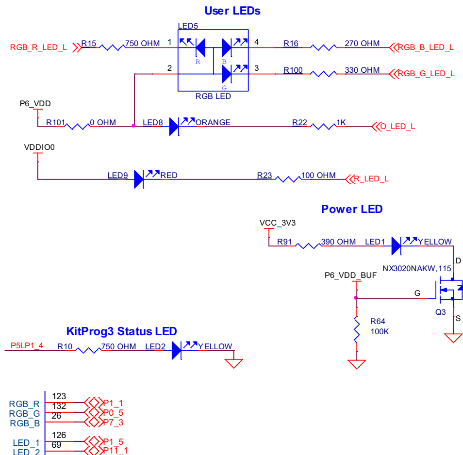
Figure 4-12. LEDs
