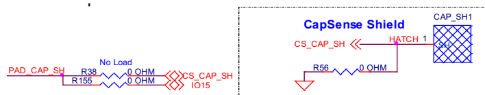
Figure 4-19. Schematics of CapSense Shield
