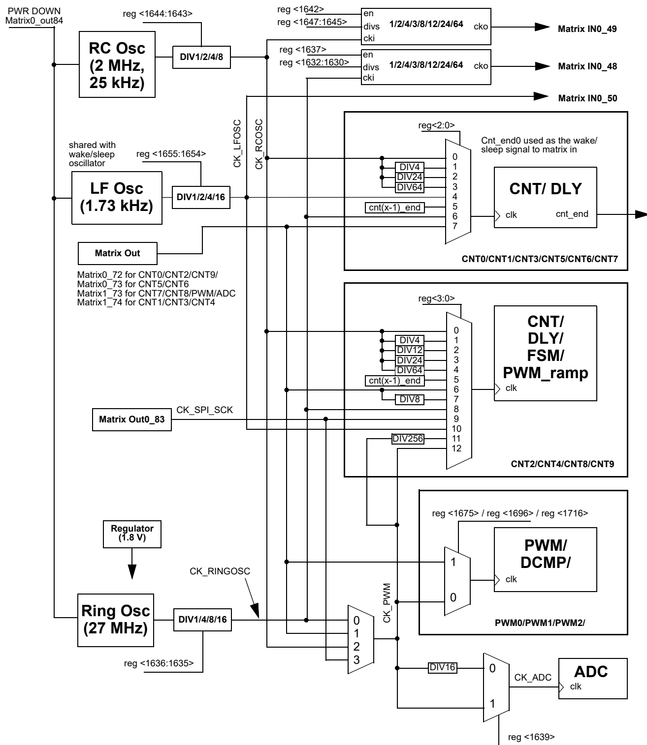
Figure 112. Oscillator Block Diagram
