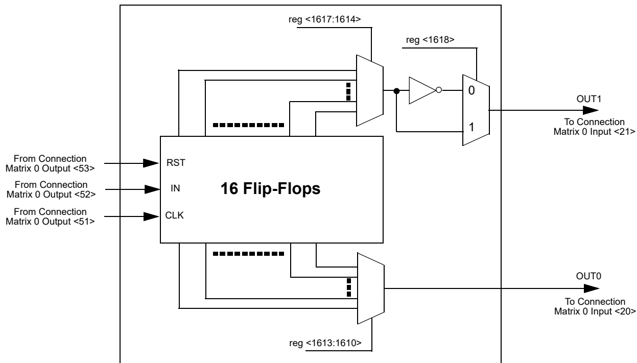
Figure 104. Pipe Delay 0
