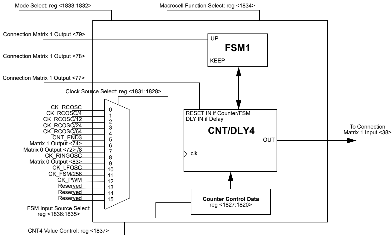
Figure 79. CNT/DLY4/FSM1
