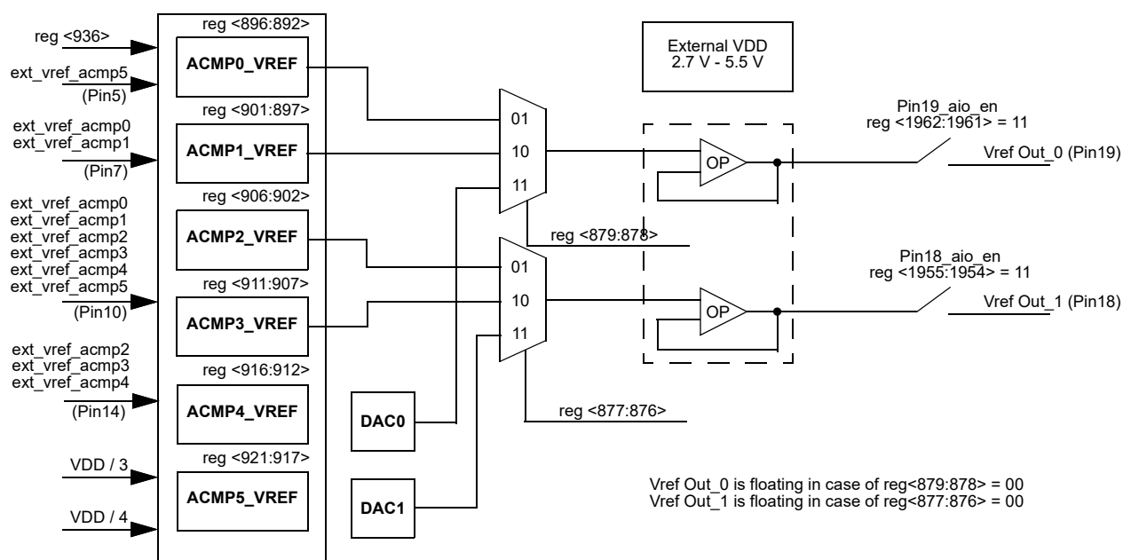
Figure 111. Voltage Reference Block Diagram
