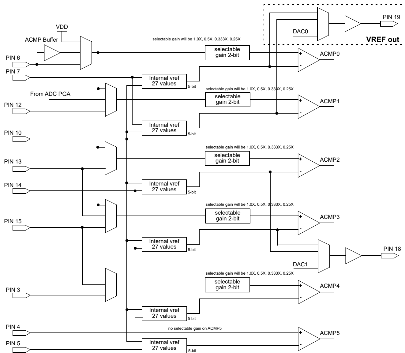
Figure 53. ACMP Master Architecture Diagram
