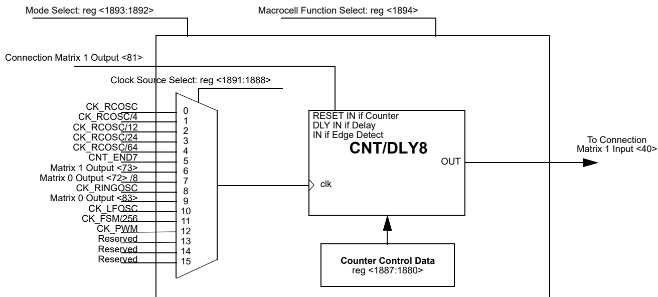
Figure 83. CNT/DLY8/PWM_RAMP
