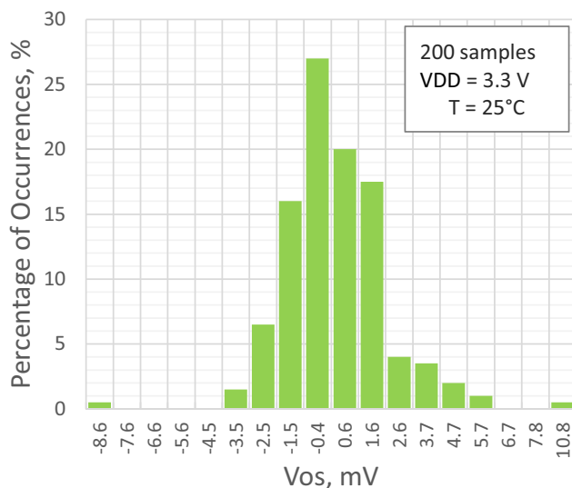
Figure 15. PGA Input Offset Distribution, Single-Ended Mode, G = 1
