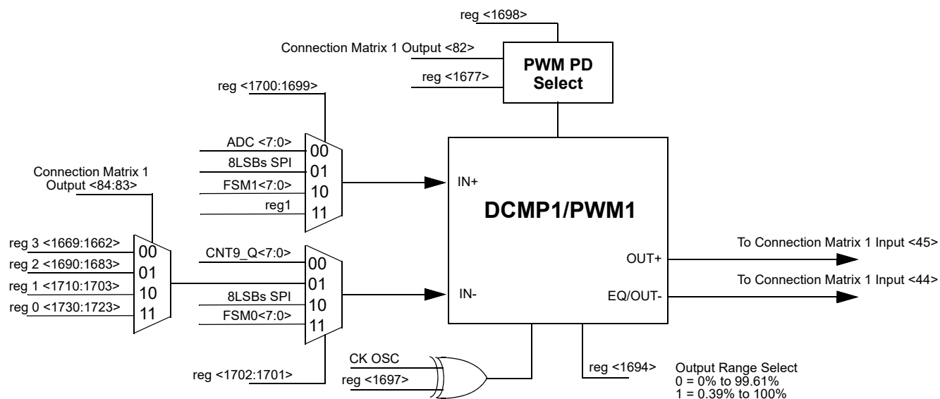
Figure 96. DCMP1/PWM1 Functional Diagram
