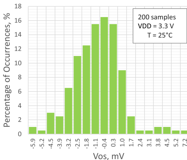
Figure 16. PGA Input Offset Distribution, Single-Ended Mode, G = 2
