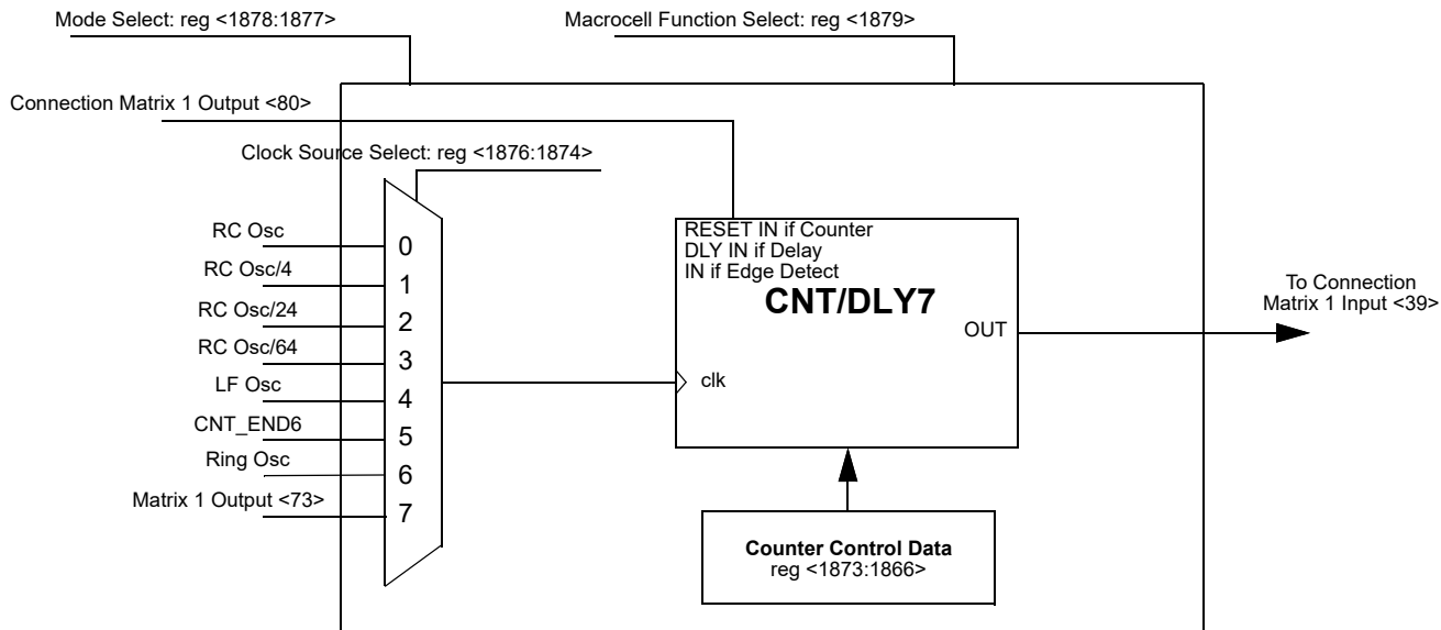
Figure 82. CNT/DLY7
