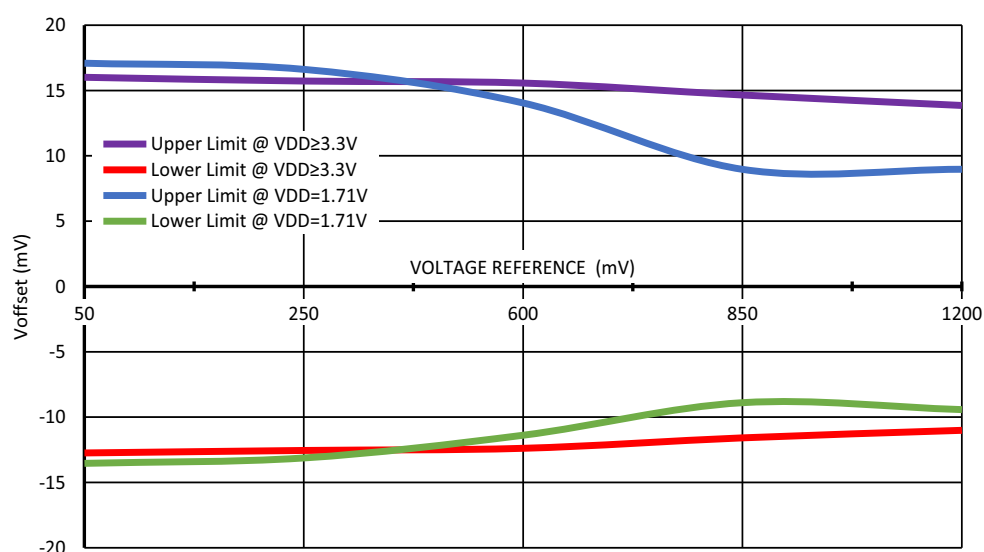
Figure 51. Buffer Input Voltage Offset vs. Voltage Reference at T = (-40.... +85)^{\circ}\text{C} , Buffer Bandwidth = 50 kHz, V_{\text{hys}} = 0 \text{ mV} , Gain = 1
