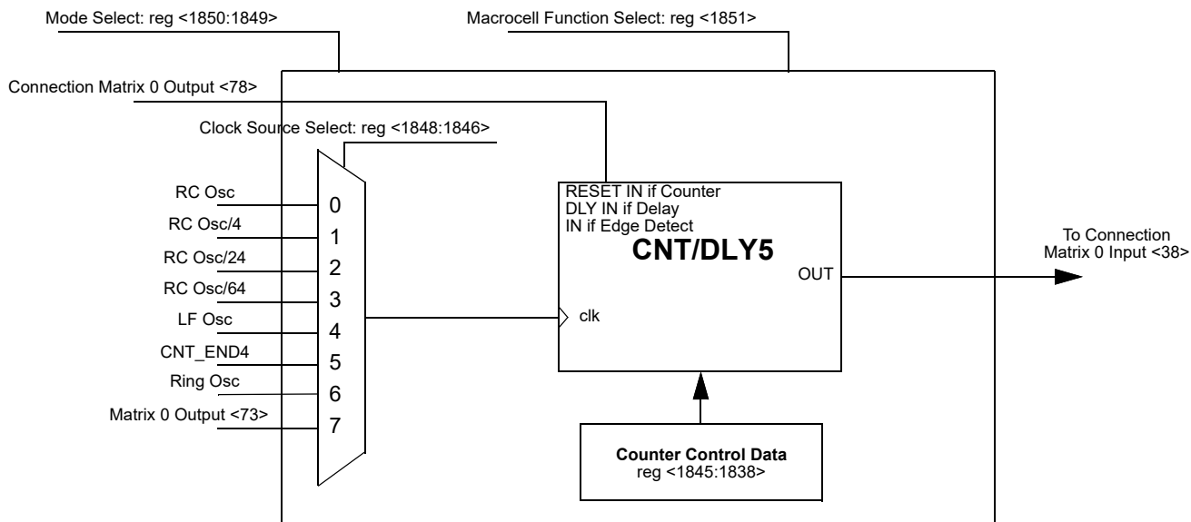
Figure 80. CNT/DLY5
