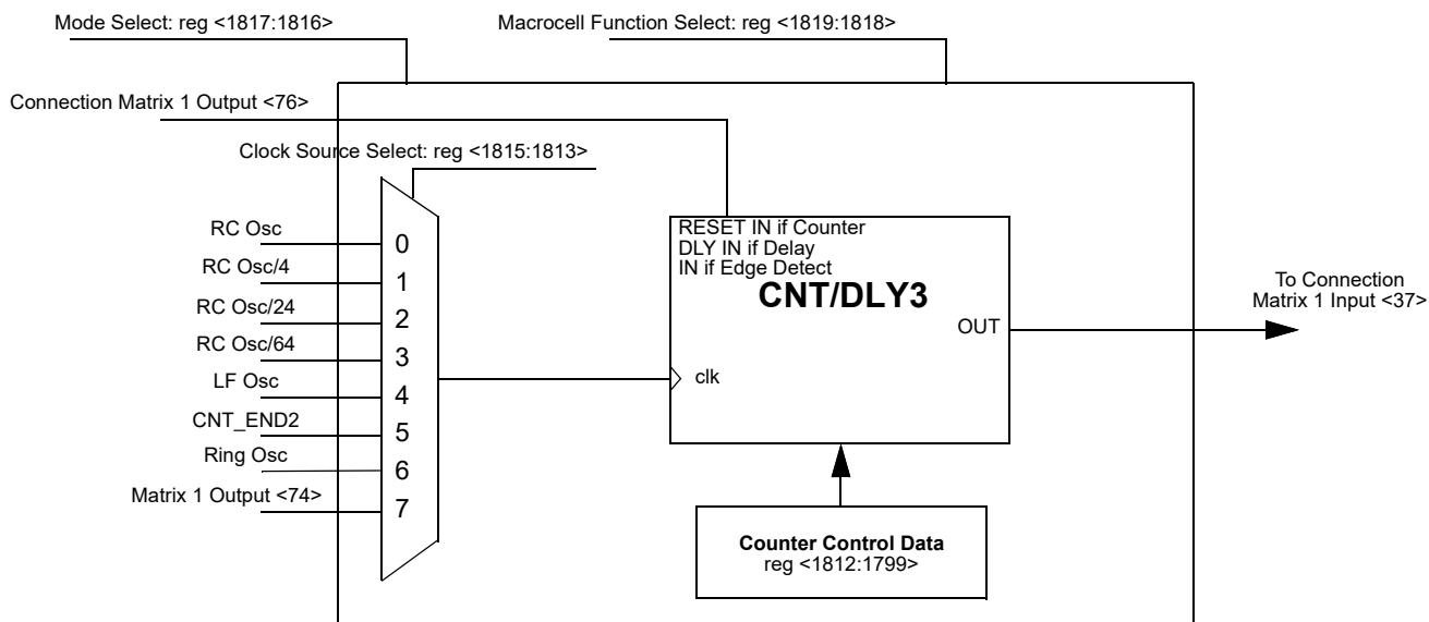
Figure 78. CNT/DLY3
