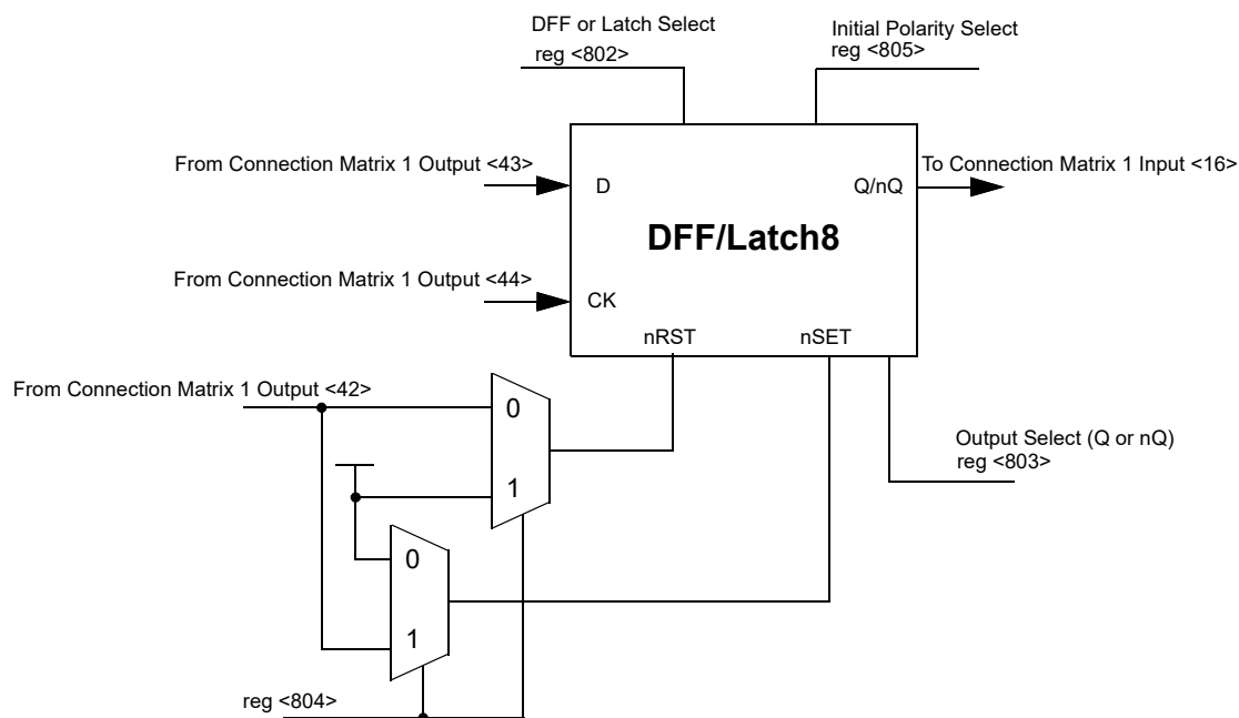
Figure 68. DFF/Latch8
