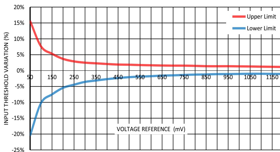
Figure 52. Input Threshold Variation (including V_{\text{ref}} variation, ACMP offset) vs. Voltage Reference at T = (-40.... +85)^{\circ}\text{C} , V_{\text{hys}} = 0 \text{ mV} , V_{\text{DD}} > 1.8 \text{ V}
