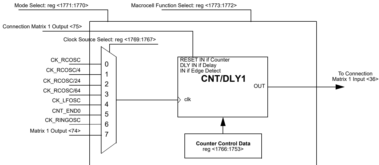
Figure 76. CNT/DLY1
