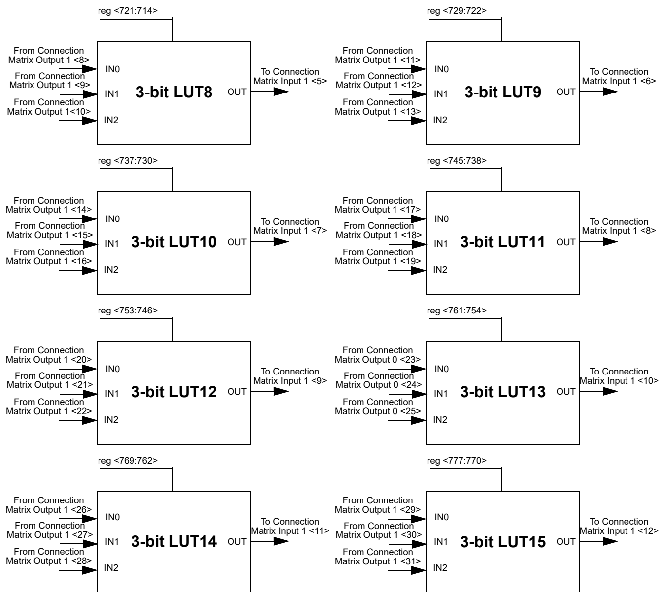
Figure 42. 3-bit LUTs
