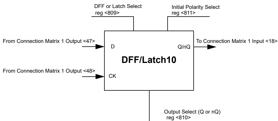
Figure 70. DFF/Latch10
