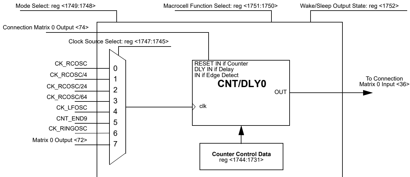
Figure 75. CNT/DLY0
