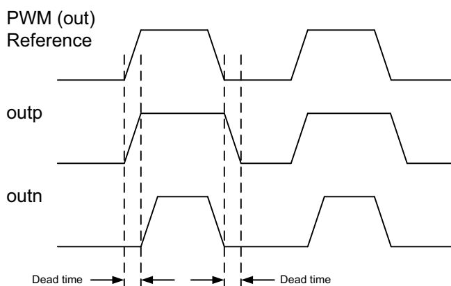
Figure 98. PWM Dead Band Control Timing Diagram
