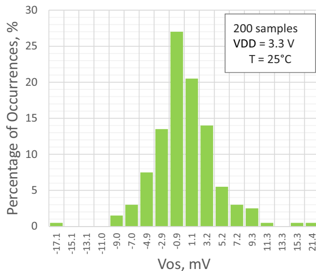
Figure 14. PGA Input Offset Distribution, Single-Ended Mode, G = 0.5
