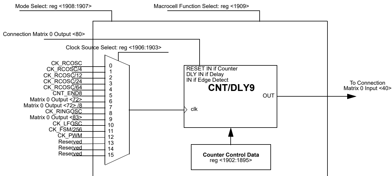
Figure 84. CNT/DLY9/PWM_RAMP
