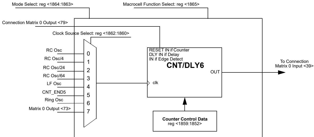
Figure 81. CNT/DLY6
