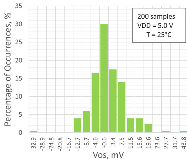
Figure 13. PGA Input Offset Distribution, Single-Ended Mode, G = 0.25
