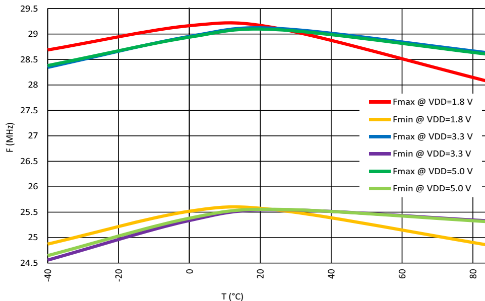
Figure 121. Ring Oscillator Frequency vs. Temperature, Ring OSC = 27 MHz
