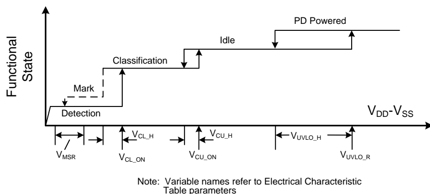
Figure 16. Threshold Voltages
