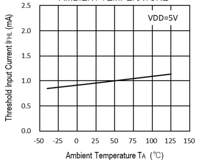
THRESHOLD INPUT CURRENT vs. AMBIENT TEMPERATURE
