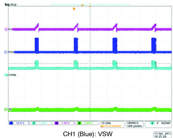
Figure 18. Typical Short Circuit Waveforms (V in = 12 V)
