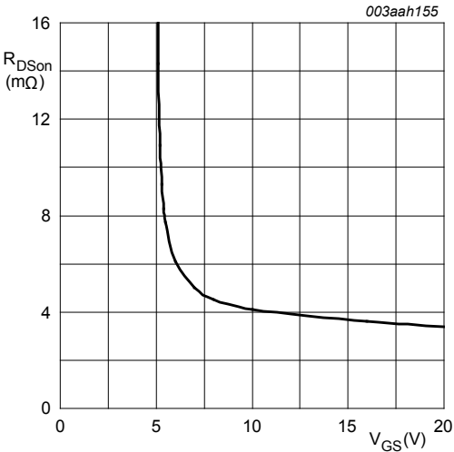
Fig. 7. Drain-source on-state resistance as a function of gate-source voltage; typical values T_j = 25\text{ }^{\circ}\text{C}; I_D = 25\text{ A}
