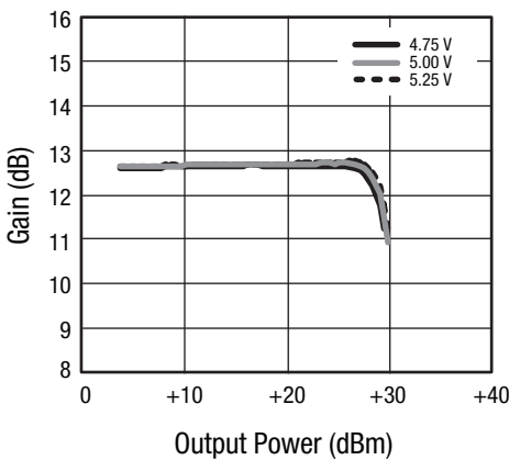
Figure 53. Gain vs Output Power Over Voltage
