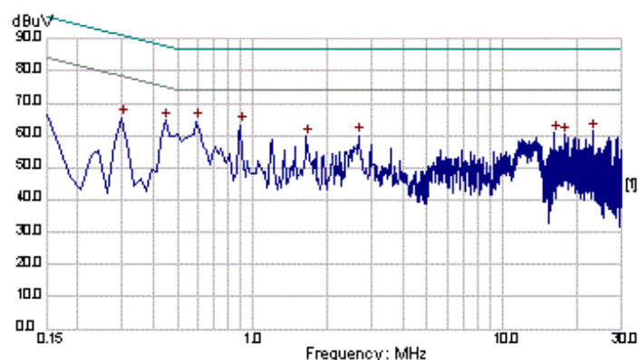
Graph 1. Conducted emissions performance, CISPR 22, Class B, full load
