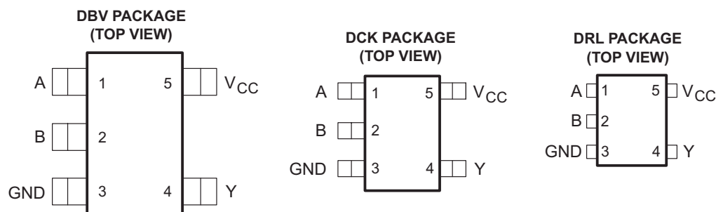
Pin Functions
