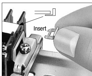
To Secure the Marking Strip
