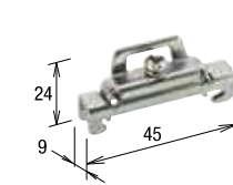
BNL6 (M4 Screw) Tightening torque: 1.1 N·m
