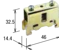
BNL8 (M4 Screw) (*3)
