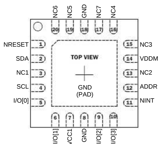
Figure 1 – SX1504 QFN-UT-20 Pinout
