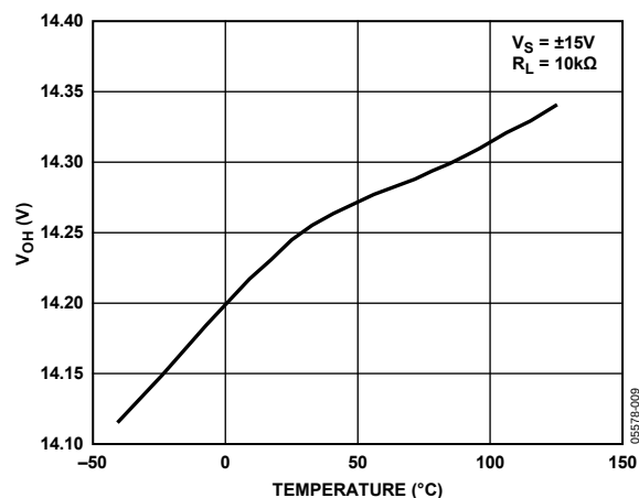
Figure 10. +V_{OUT} vs. Temperature
