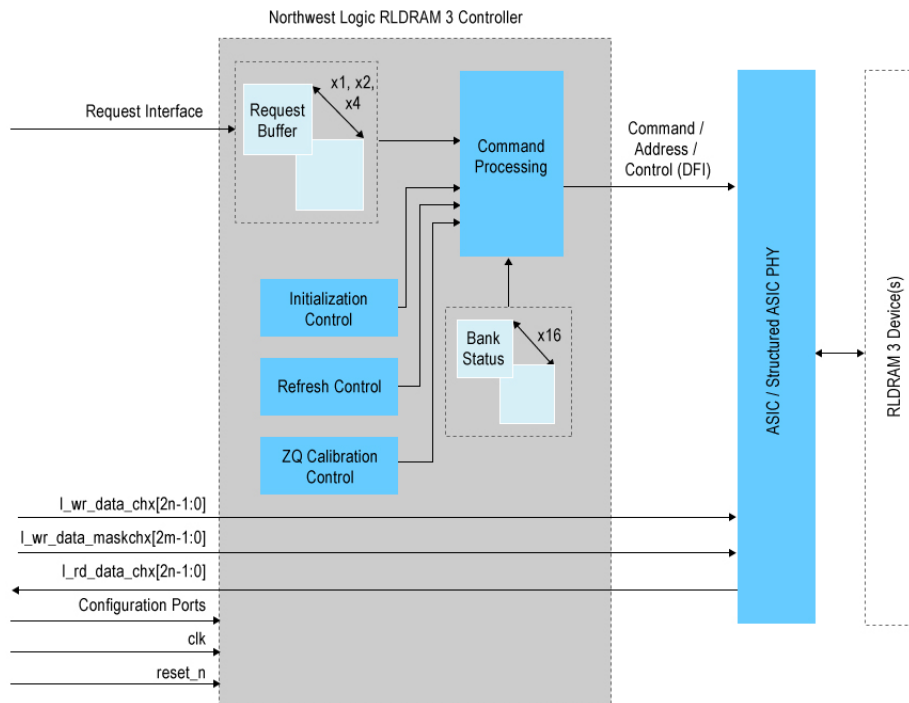
Figure 14. RLDAM3 Block Diagram
