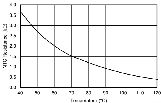
Figure 7-12. NTC Sensor Resistance vs Temperature
