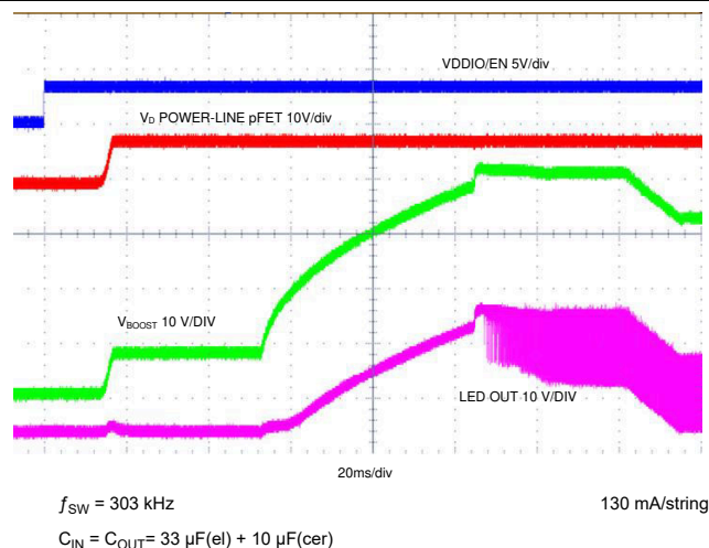
Figure 7-5. Typical Start-up
