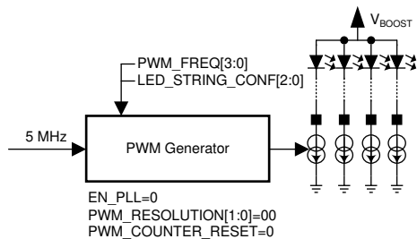
Figure 6-2. PWM Clocking With Internal Oscillator
