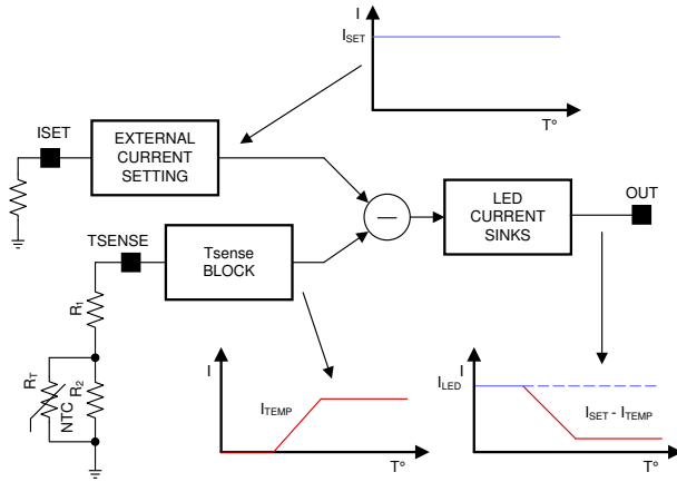
Figure 6-27. Temperature-Dependent NTC Current (Subtracted from ISET Current)
