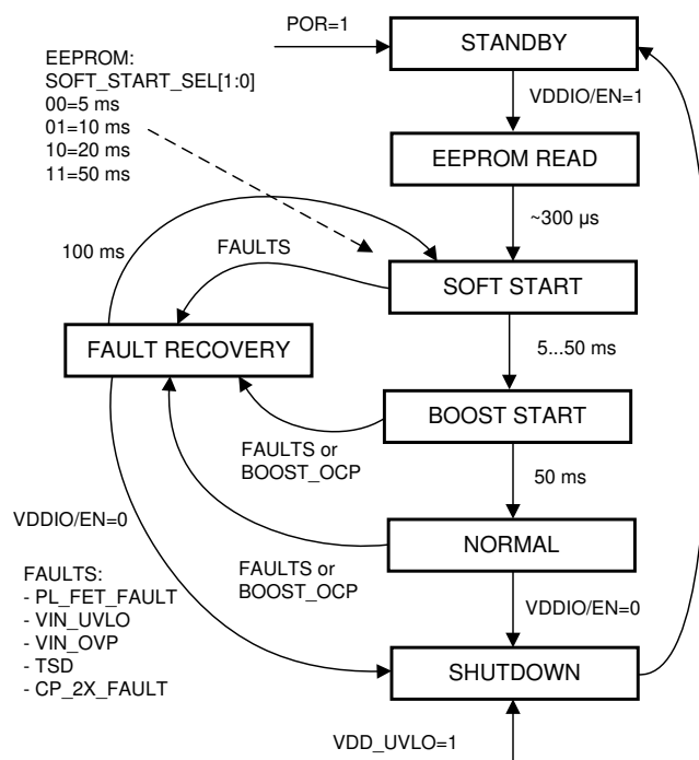
Figure 6-34. State Diagram
