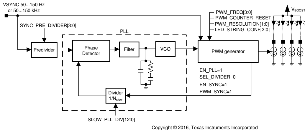
Figure 6-4. PWM Synchronization With External VSYNC Input
