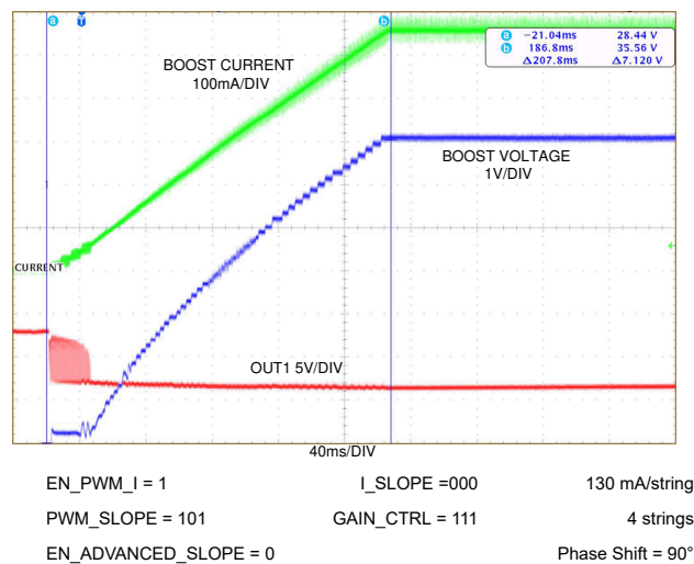
Figure 7-7. Slope With Hybrid Dimming and Phase Shift
