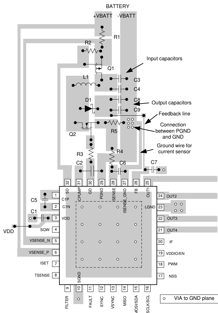
Figure 7-15. LP8860-Q1 Layout
