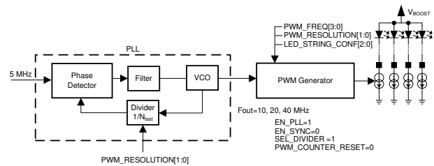
Figure 6-3. PWM Clocking With PLL, Internal Oscillator as Reference
