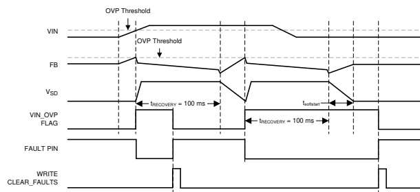
Figure 6-29. Input OVP Triggering and Recovery
