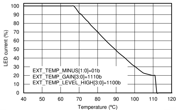
Figure 7-13. LED Current De-rating vs Temperature
