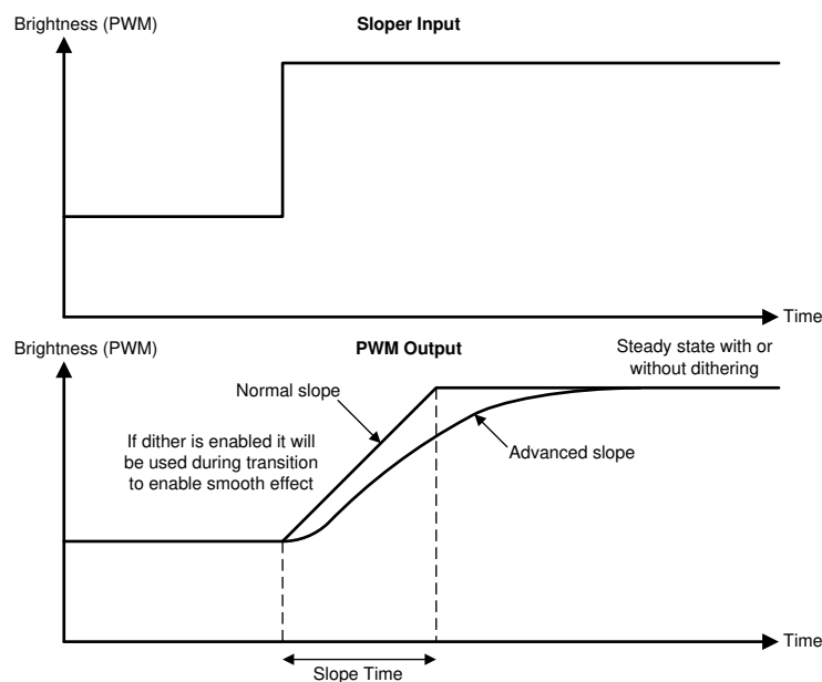
Figure 6-6. Sloper Operation
