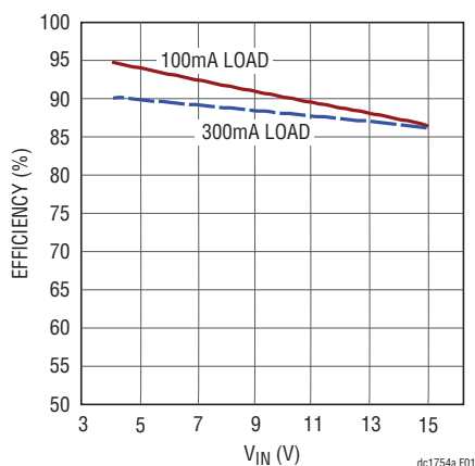
Figure 1. DC1754A Efficiency in PWM Mode
