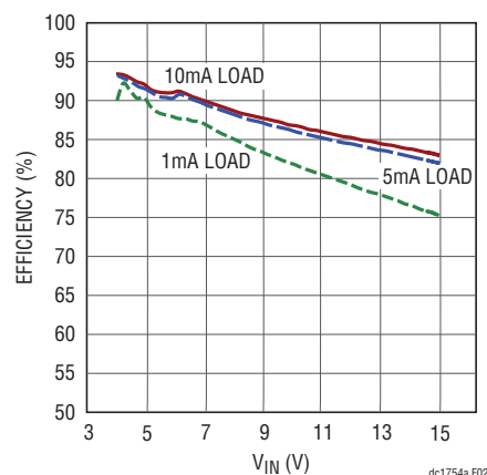
Figure 2. DC1754A Efficiency in Burst Mode Operation
