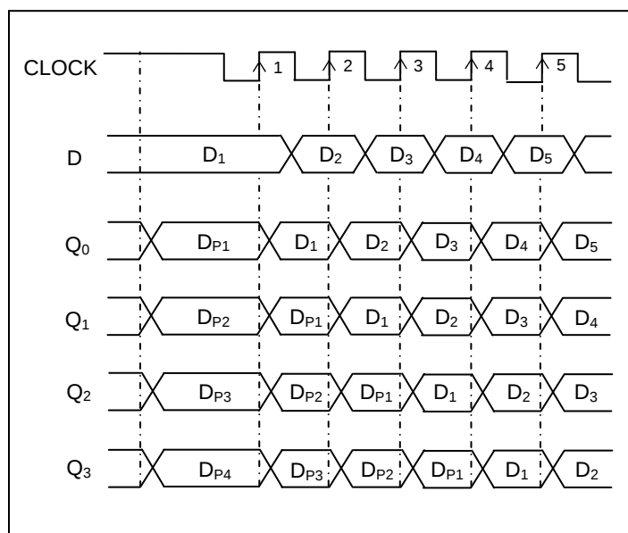
Timing Chart
