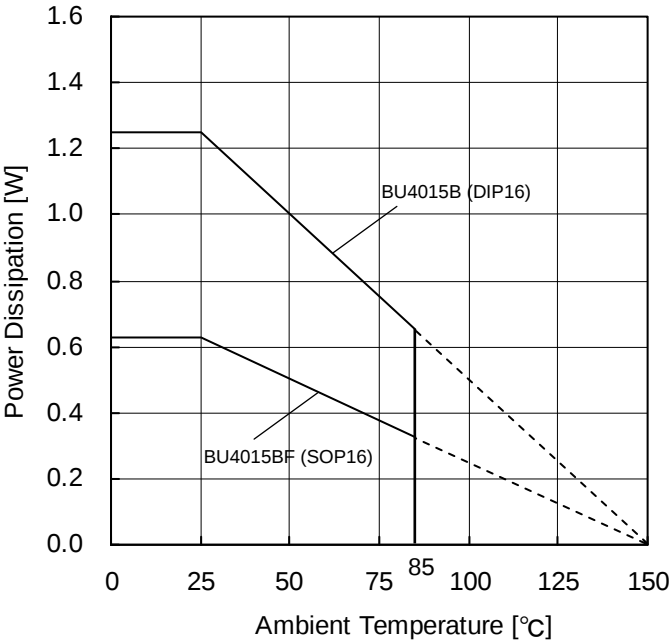
Figure 11. Derating Curve
