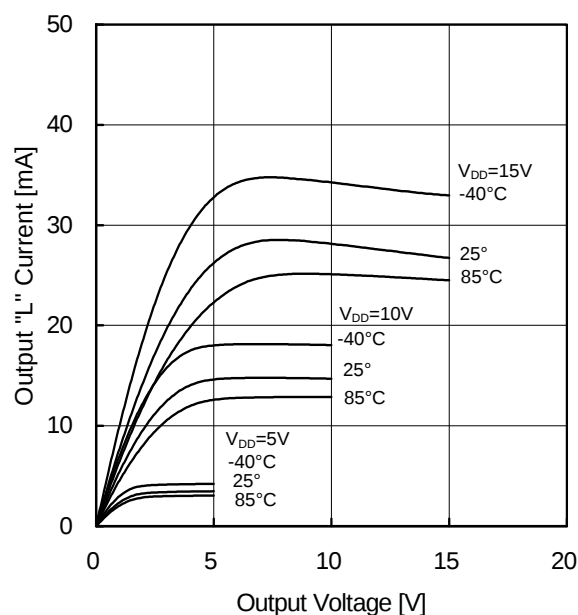
Figure 2. Output "L" Current vs Output Voltage
