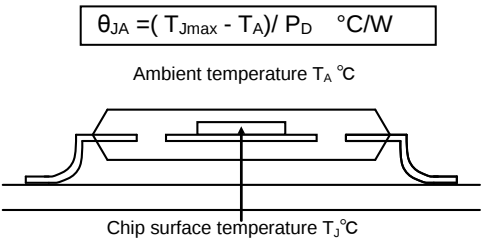
Figure 10. Thermal resistance
