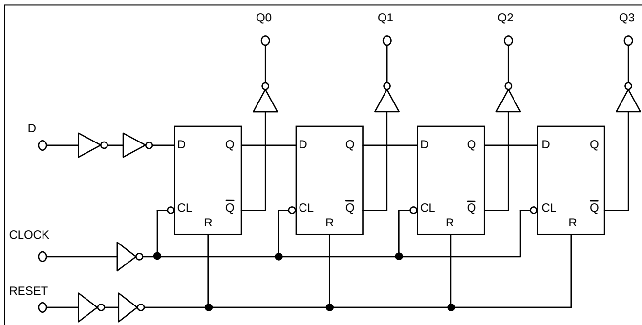
Logic Diagram
