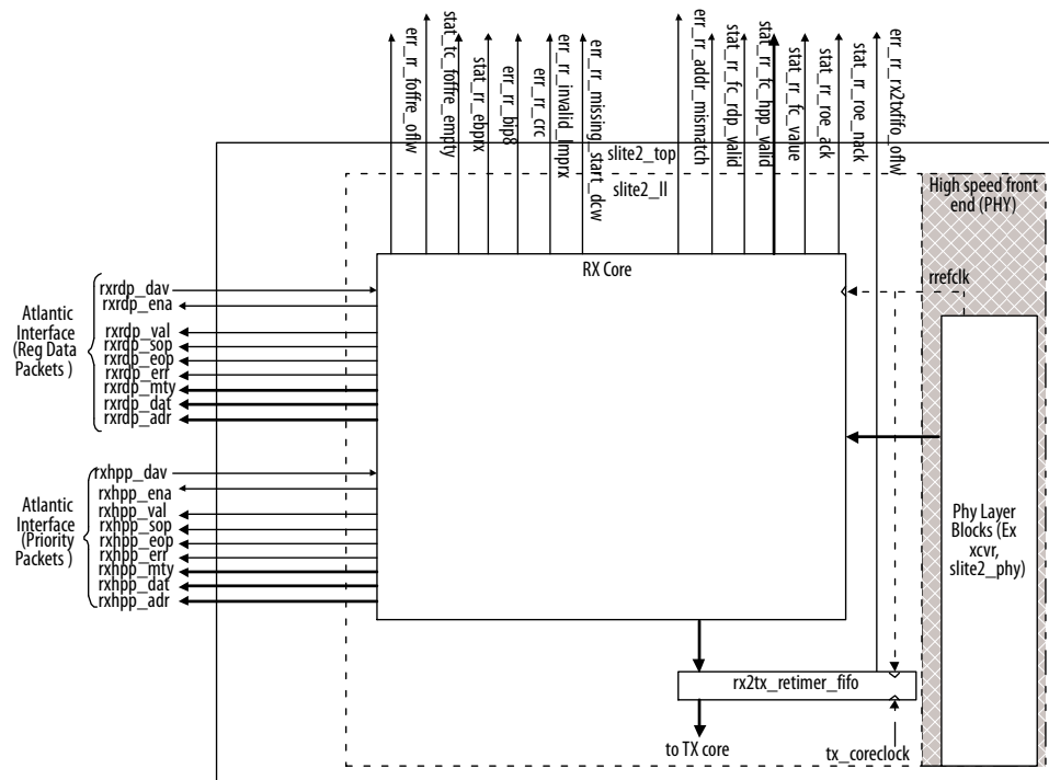
Figure 28. Receiver Layer With No FIFO
