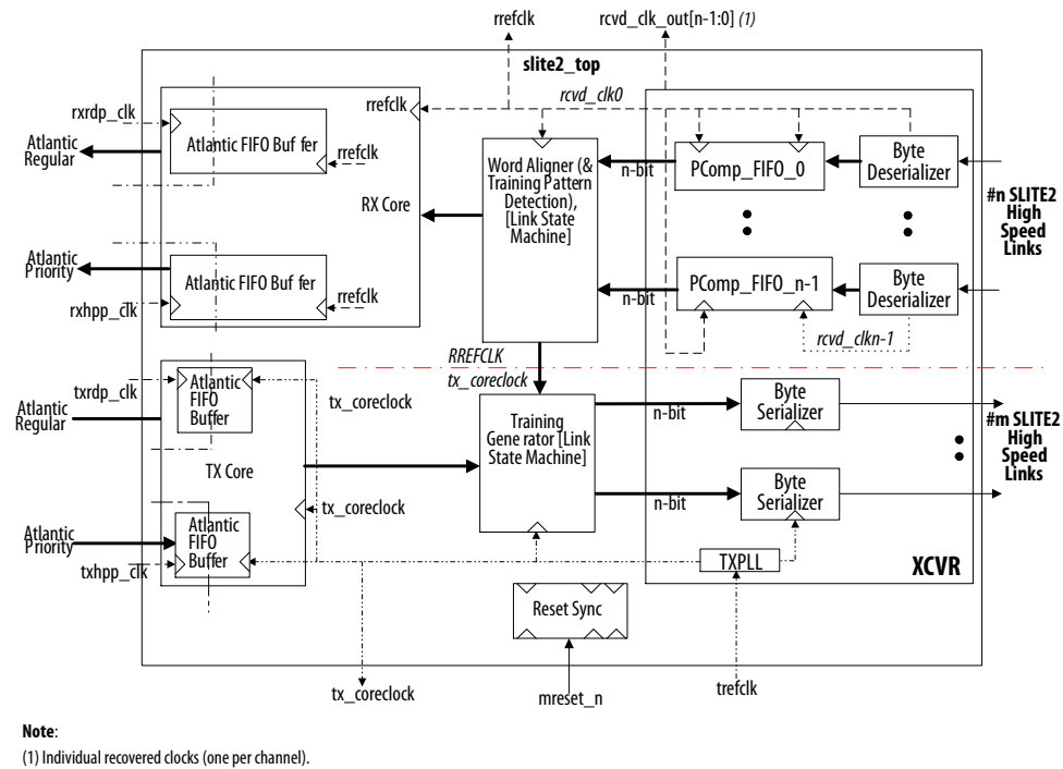
Figure 23. No Receiver FIFO Buffers No Frequency Offset Clock Structure
