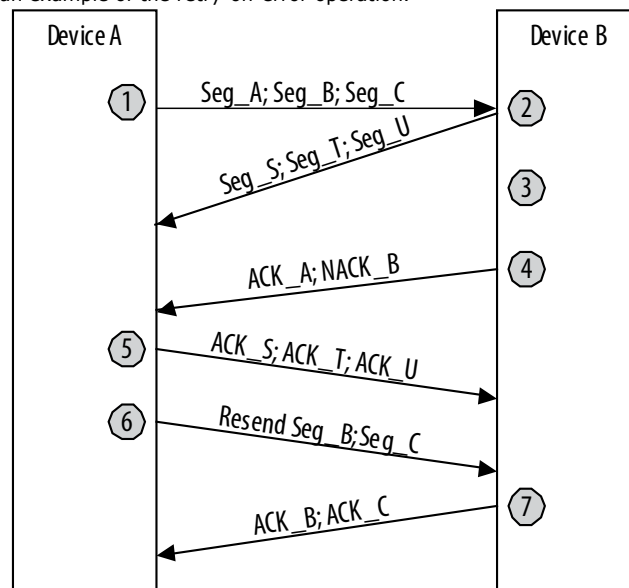
Figure 13. Retry-On-Error Example
